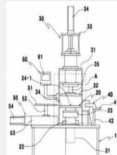
Induction Heating Coil Compression Wiring Device
